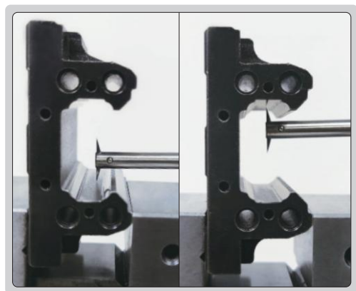
slider
