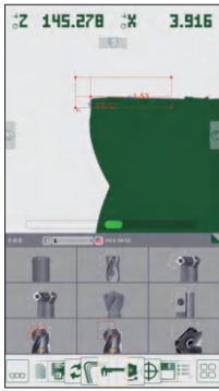
fast measurement, automatic recognition of cutting edge shapes
