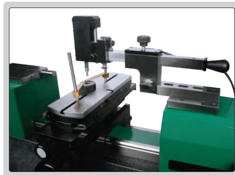
thread ring gauge measurement
