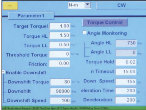
interface of tightening parameter setting
